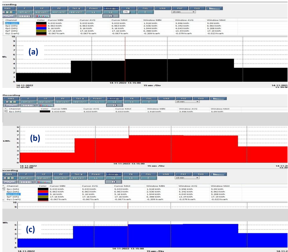
Figure 4.4 Energy Generated by 500 KVA DG Set on trial – (a) Phase-1, (b) Phase-2, and (c) Phase-3.
