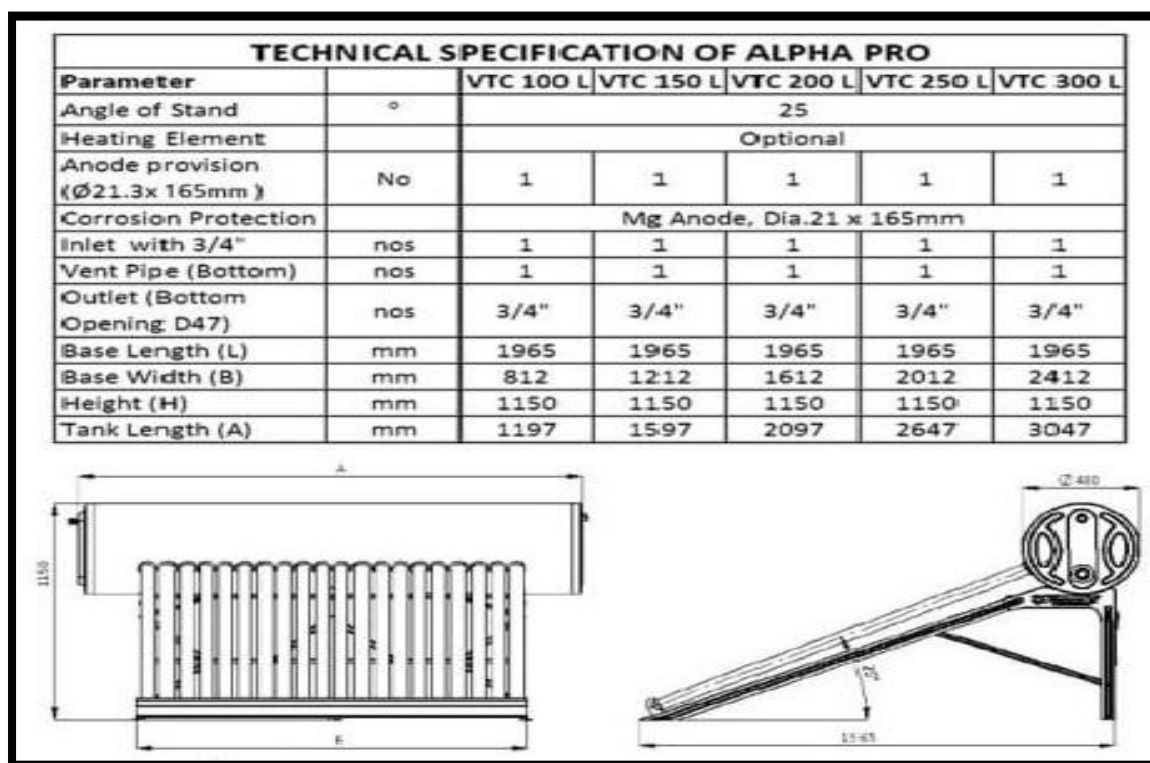
Figure 4-7 Technical specifications of solar water boiler
