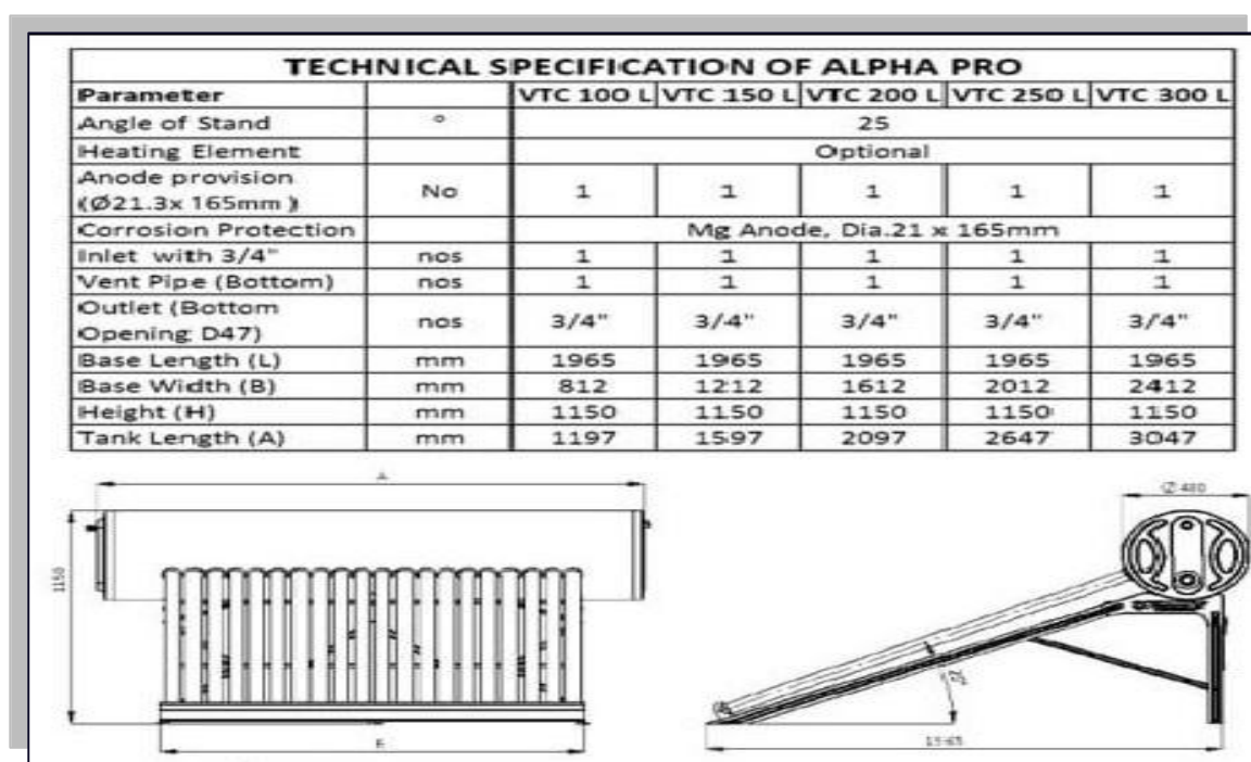
Figure 4-7 Technical specifications of solar water boiler
