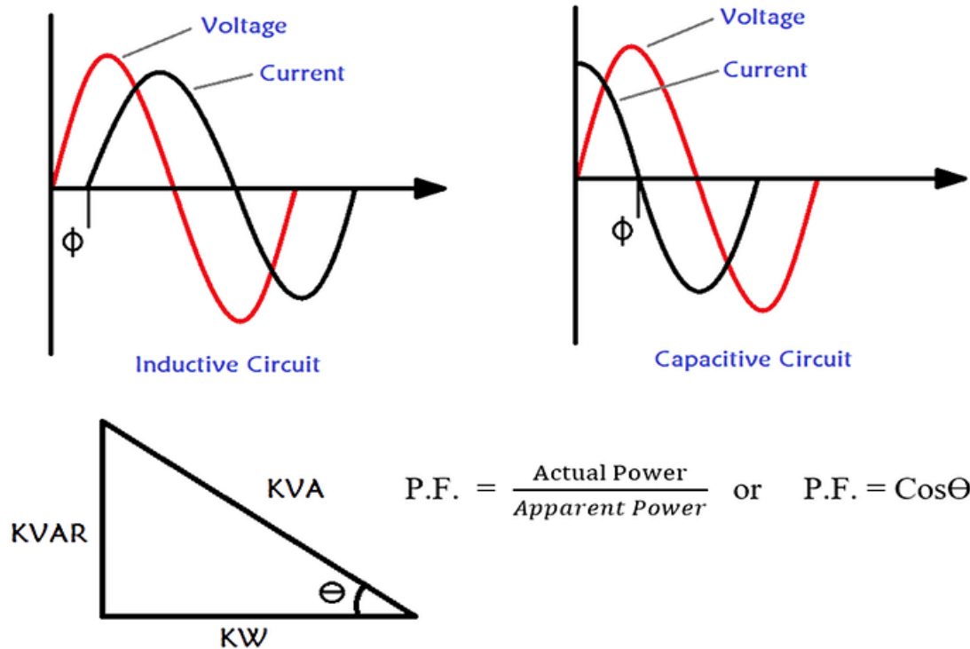
Figure 4-19 Power Factor Waveform
