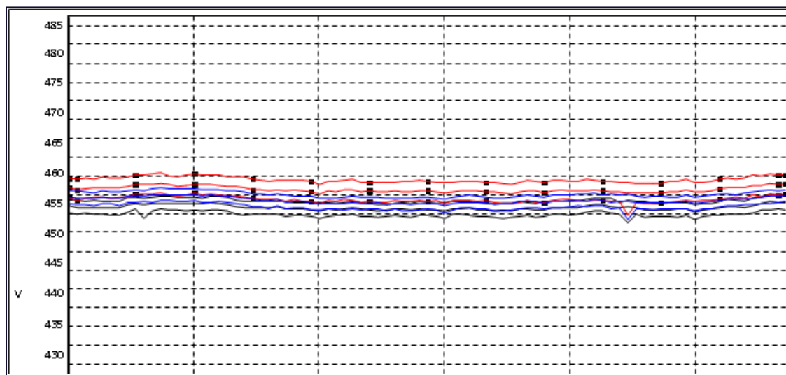
Figure 4-10 voltage graph of 1250KVA transformer 2
